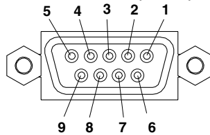
Pin arrangement of the EXT I/O terminal (female)
