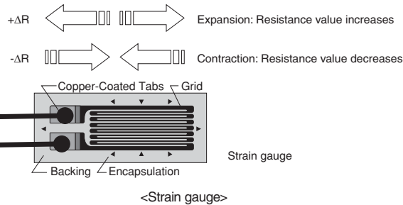
<Strain gauge>
