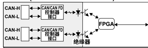
720242 (CAN/CAN FD MONITOR)
