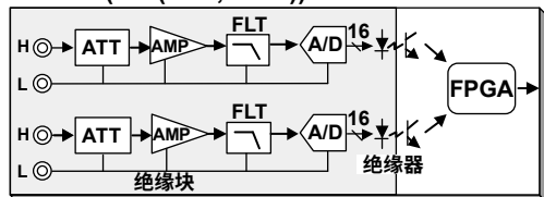
720268 (HV (AAF, RMS))
