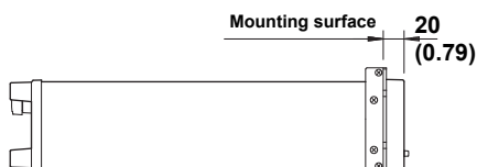
EIA rack mount dimensions
