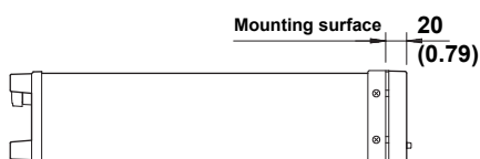
EIA rack mount dimensions
