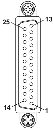
Pin arrangement
