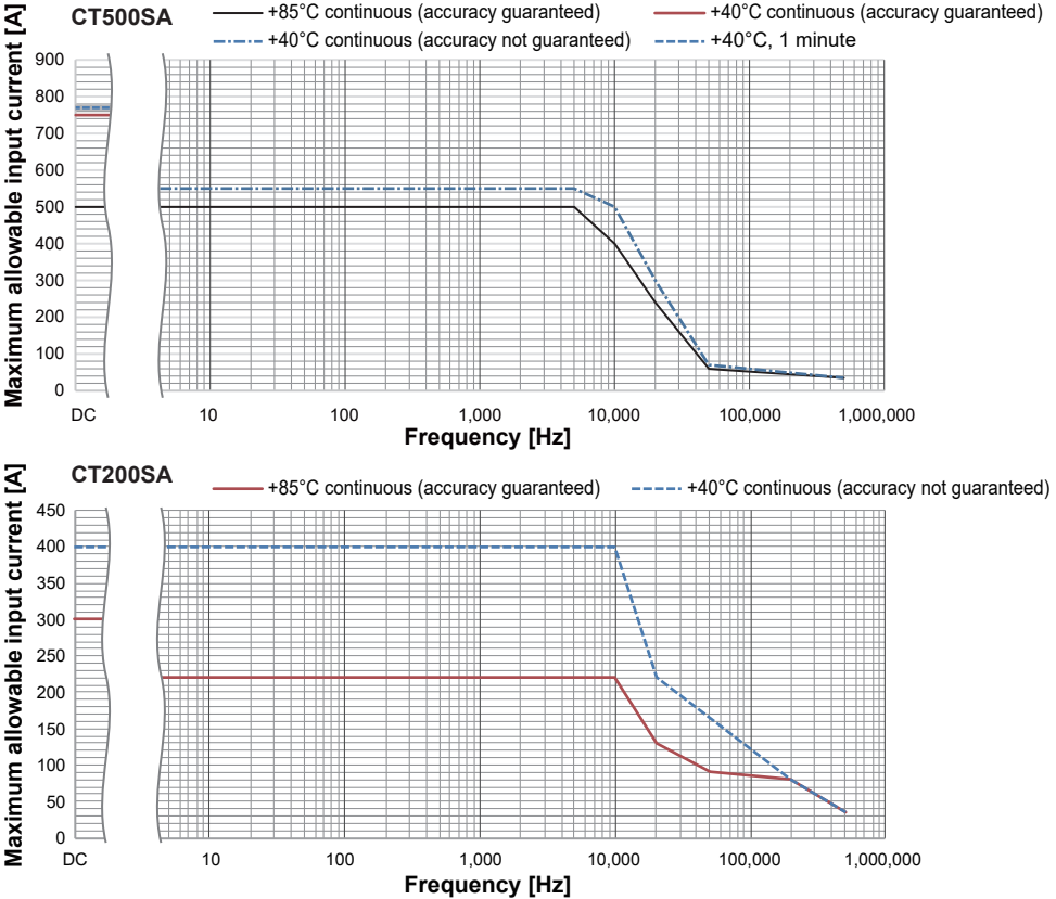
Figure 2. Input current derating by frequency* * The derating characteristics are specified with no external magnetic field present and with the conductor centered. The temperatures shown in the figure are the maximum operating ambient temperatures. (Make sure that the surface temperature of the conductor under test is within the instrument's operating ambient temperature range.)
