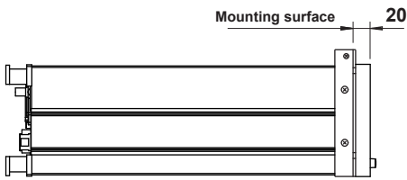
JIS rack mount dimensions
