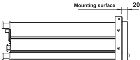
EIA rack mount dimensions
